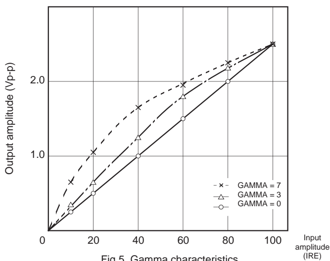
Fig 5. Gamma characteristics
